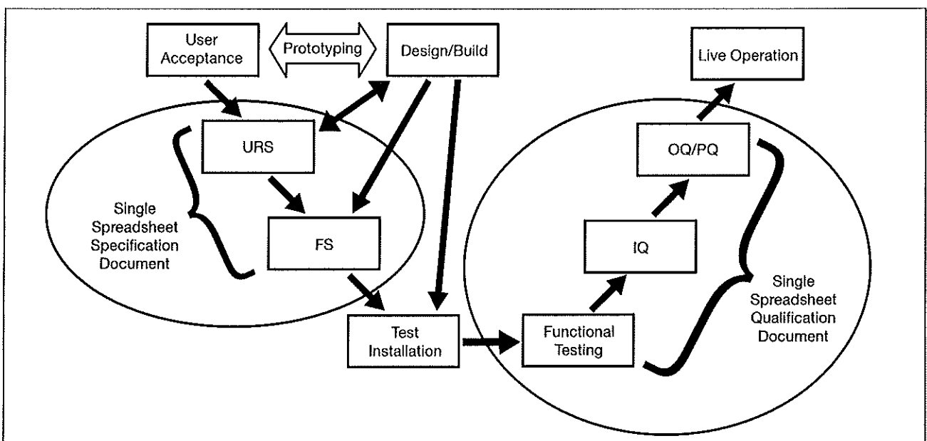
Figure 1: Amended V model for Excel Spreadsheet Validation
